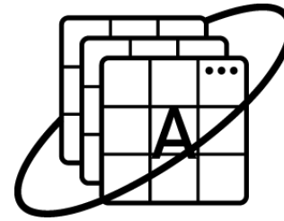
Containers & microservices
