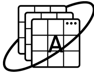
Modern apps
